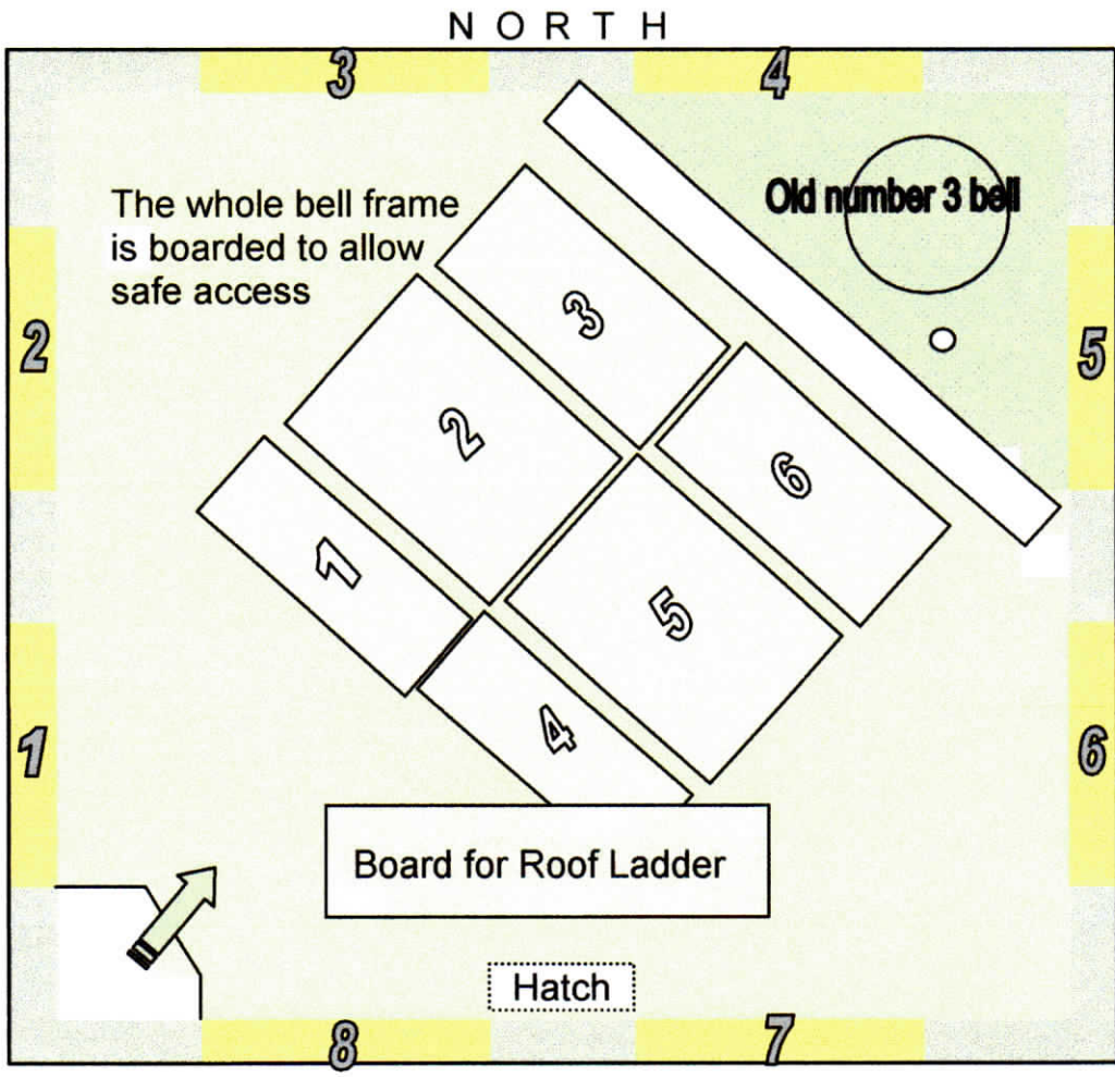
DIAGRAM OF THE SHUTTER DOORS AND LOOSE LAID HATCHES IN THE OLD BELFRY
